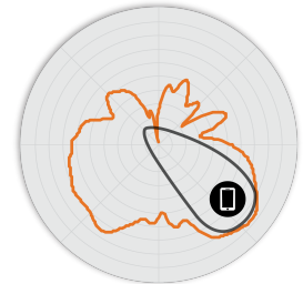
Figure 7. R770 6GHz Elevation Antenna Patterns
