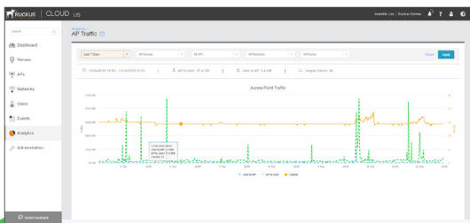
Figure 3: AP Traffic
